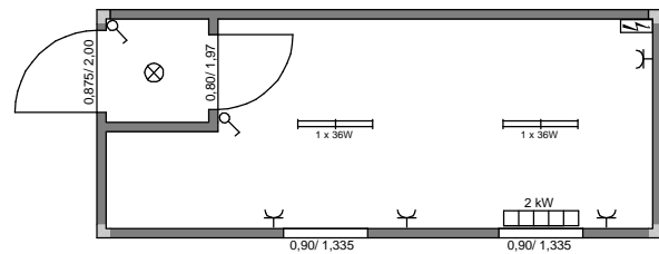
ARS E 21 - (LxB) 6,058m x 2,438m; RH = 2,50m
